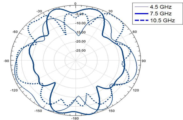
Fig. 4. The normalized antenna radiation pattern for a set of frequencies
