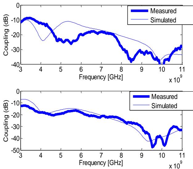
Fig. 13. The antenna coupling for both positions
