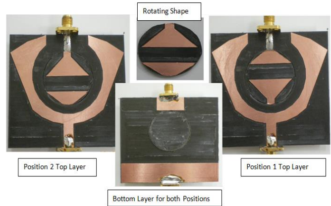
Fig. 10. The fabricated antenna prototype
