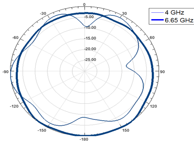
Fig. 8. The normalized radiation pattern for position 1 and 2
