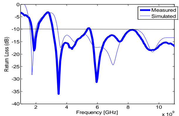
Fig. 11. The "sensing" antenna return loss
