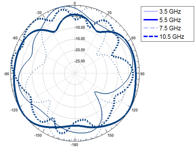
Fig. 14. The normalized antenna radiation pattern
