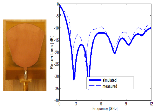
Fig. 1. The antenna structure and its return loss
