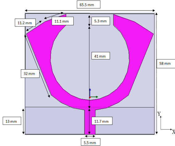
Fig. 2. The "Sensing" antenna structure
