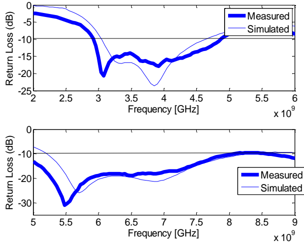
Fig. 12. The “reconfigurable communicating” return loss for both positions
