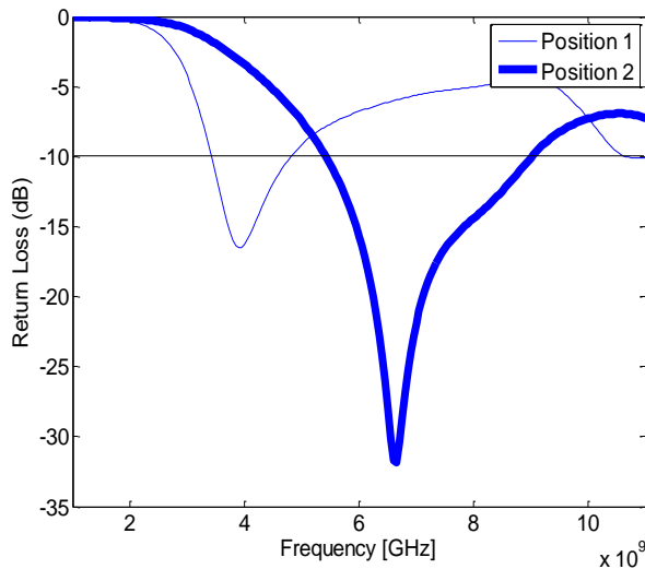
Fig. 7. Frequency tuning for the "reconfigurable communicating" antenna
