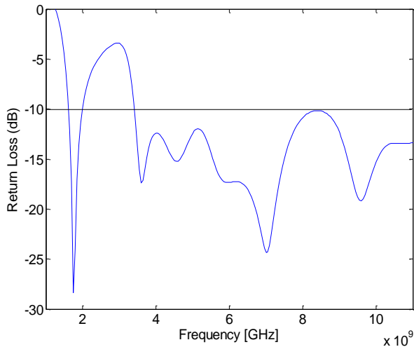
Fig. 3. The return loss for the sensing antenna structure
