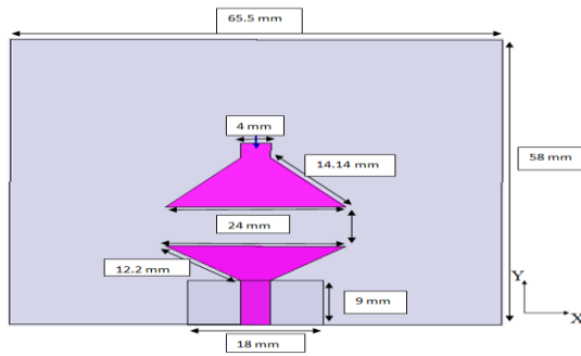
Fig. 5. The "Reconfigurable Communicating" antenna structure
