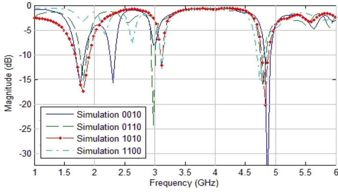
Fig. 3. Antenna resonances for different diode states: 0—OFF, 1—ON.
