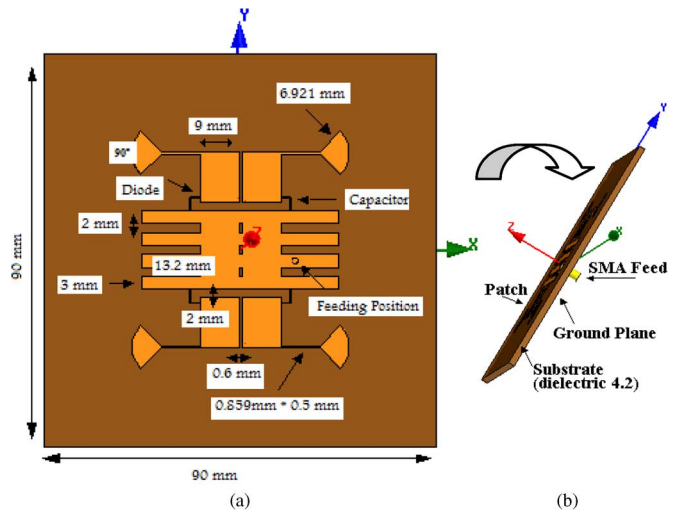
Fig. 2. (a) Front view with different dimensions. (b) Side view of the antenna.
