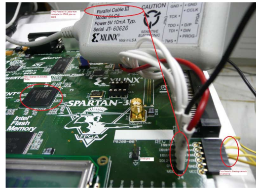
Fig. 7. The parallel III cable with FPGA board.
