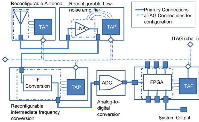
Fig. 1. Canonical reconfigurable system, based on connection of configurable and nonconfigurable components, controlled by common JTAG scan chain.
