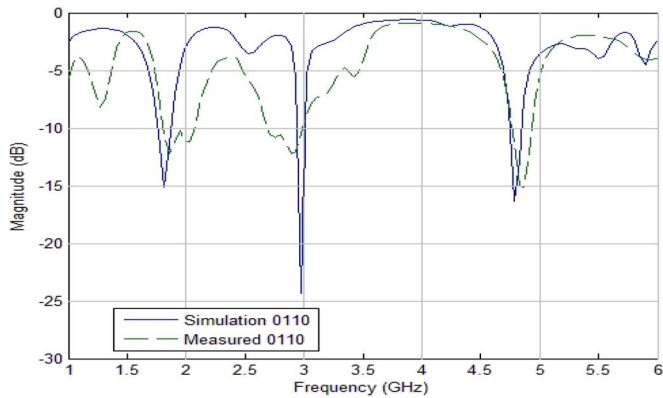
Fig. 9. Measured and simulated |S_{11}| comparison for the 0110 antenna state.
