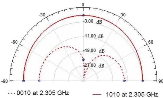
Fig. 5. Comparison between the E -plane cut ( yz ) of the simulated radiation pattern for two switch configurations at 2.305 GHz.
