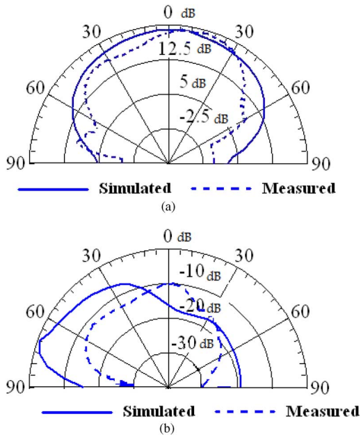
Fig. 4. Simulated and measured radiation pattern comparison at 4.875 GHz with all switches OFF: (a) E -plane cut ( yz ) and (b) H -plane cut ( xz ).
