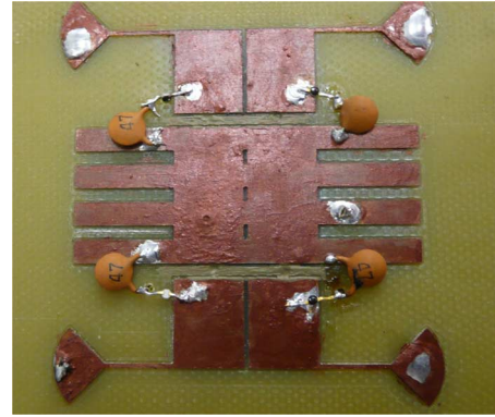
Fig. 6. Photograph of the fabricated prototype.
