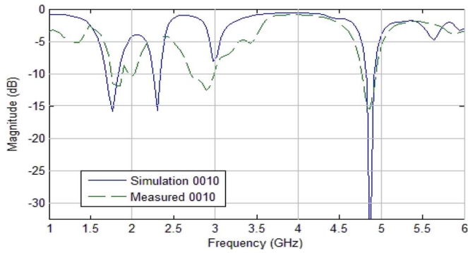
Fig. 8. Measured and simulated |S_{11}| comparison for the 0010 antenna state.
