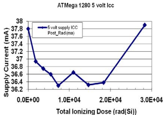
Fig. 11. ATMega 1280 post-radiation 5 volt supply current.
