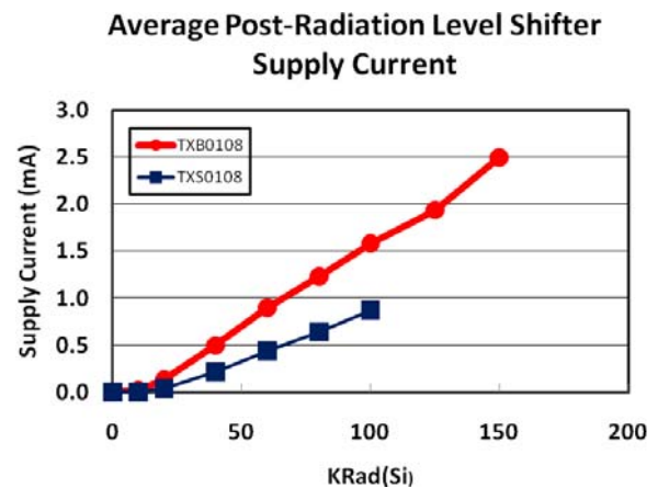
Fig. 6 Average post-irradiation supply current for TXS0108 and TXB0108
