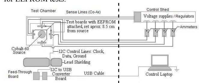
Fig. 1. Schematic of 60 Co test arrangement
