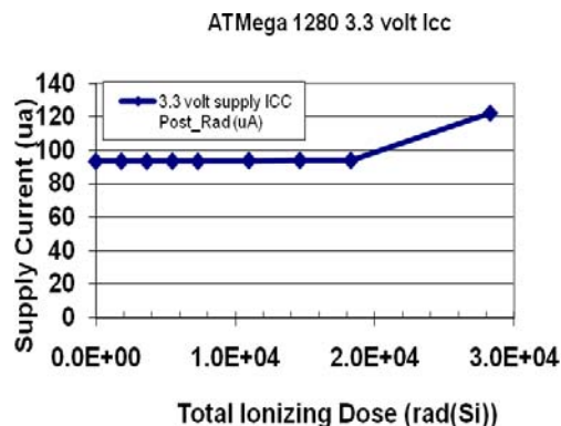
Fig. 12. ATMega 1280 post-radiation 3.3 volt supply current.
