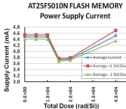
Fig. 16. AT25FS010N post-irradiation supply current
