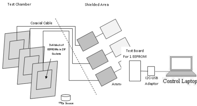
Fig. 3. Schematic for ^{137}\text{Cs} test arrangement
