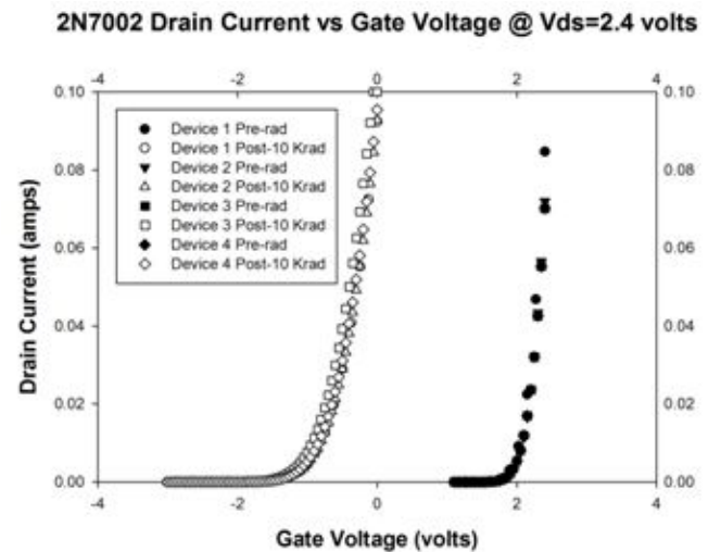
Fig. 10. 2N7002K post-irradiation (10 Krad(Si)) threshold voltage characteristic.
