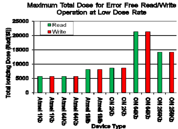
Fig. 18. Low Dose Rate Error Free Operation Summary
