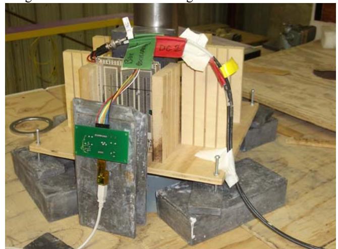
Fig. 2. Test fixture for 60 Co irradiation
