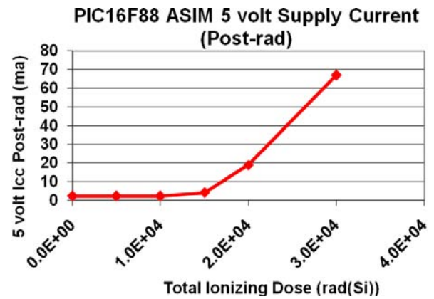
Fig. 13. PIC16F88 post-radiation 5 volt supply current
