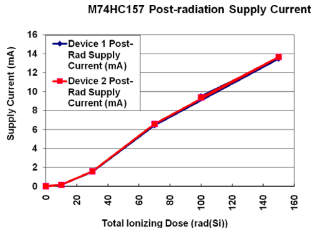
Fig. 9. 74HC157 Multiplexer post-irradiation supply current.
