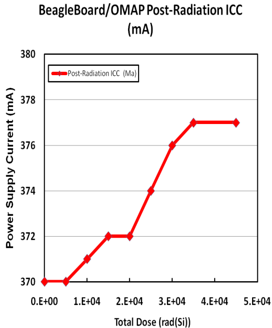
Fig. 14. BeagleBoard post-radiation 5 volt supply current
