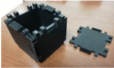
Figure 10. Six panels form 1U CubeSat.
