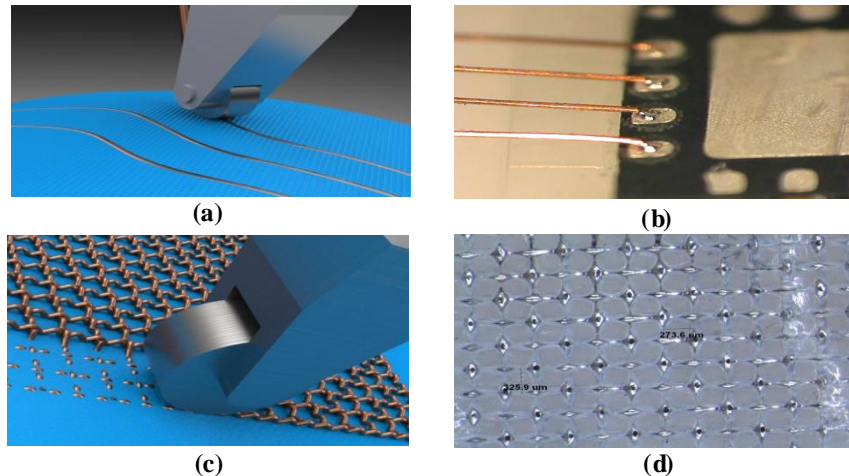
Figure 17. (a) CAD depiction of wire embedding. (b) Laser-welded component. (c) CAD depiction of embedded mesh. (d) Picture of surface after mesh embedding
