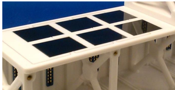
Figure 8(b). Completed 3U CubeSat prototype with embedded copper wire connecting a solar CIC array to the power bus.
